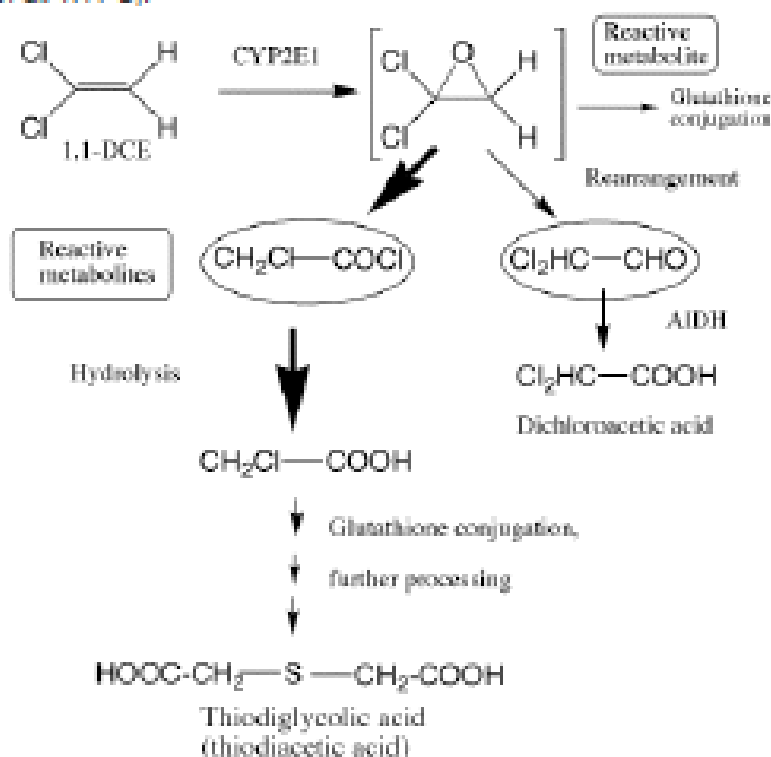
Figure 1: Metabolic pathways for 1,1-dichloroethene (1,1-DCE)
