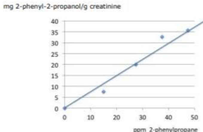
Figure 1. Mean 2-phenyl-2-propanol after experimental human exposure to 2-phenylpropane (experiment of Knecht and Ulshöfer 1996; linear function forced through the origin).
